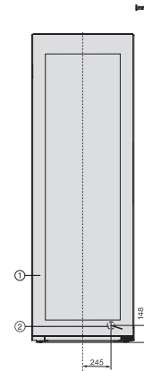
KWTS4785F obsw, Rioja, installation (footnote*) (installation drawings)
